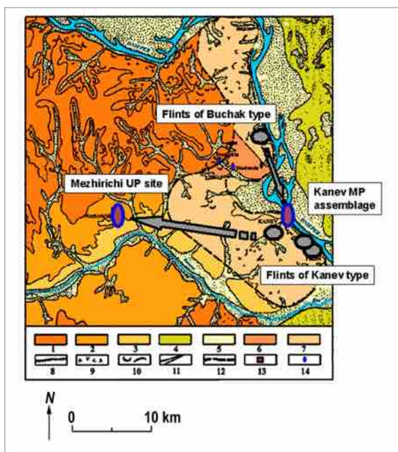
Fig. 4. Kanev area: outcrops, Palaeolithic localities, and probable connections between the two. Key: 1 – plateau, 2 – moraine terraces, 3 – loess terrace, 4 – I terrace (sand), 5 – fluvial terrace, 6 – dislocated plateau, 7 – dislocated moraine terrace, 8 – bank incuts, 9 – working ravines, 10 – displacements, 11 – passing valleys, 12 – borders of Kanev dislocations, 13 – stratigraphic sections with Kanev flints, 14 – Palaeolithic localities.
